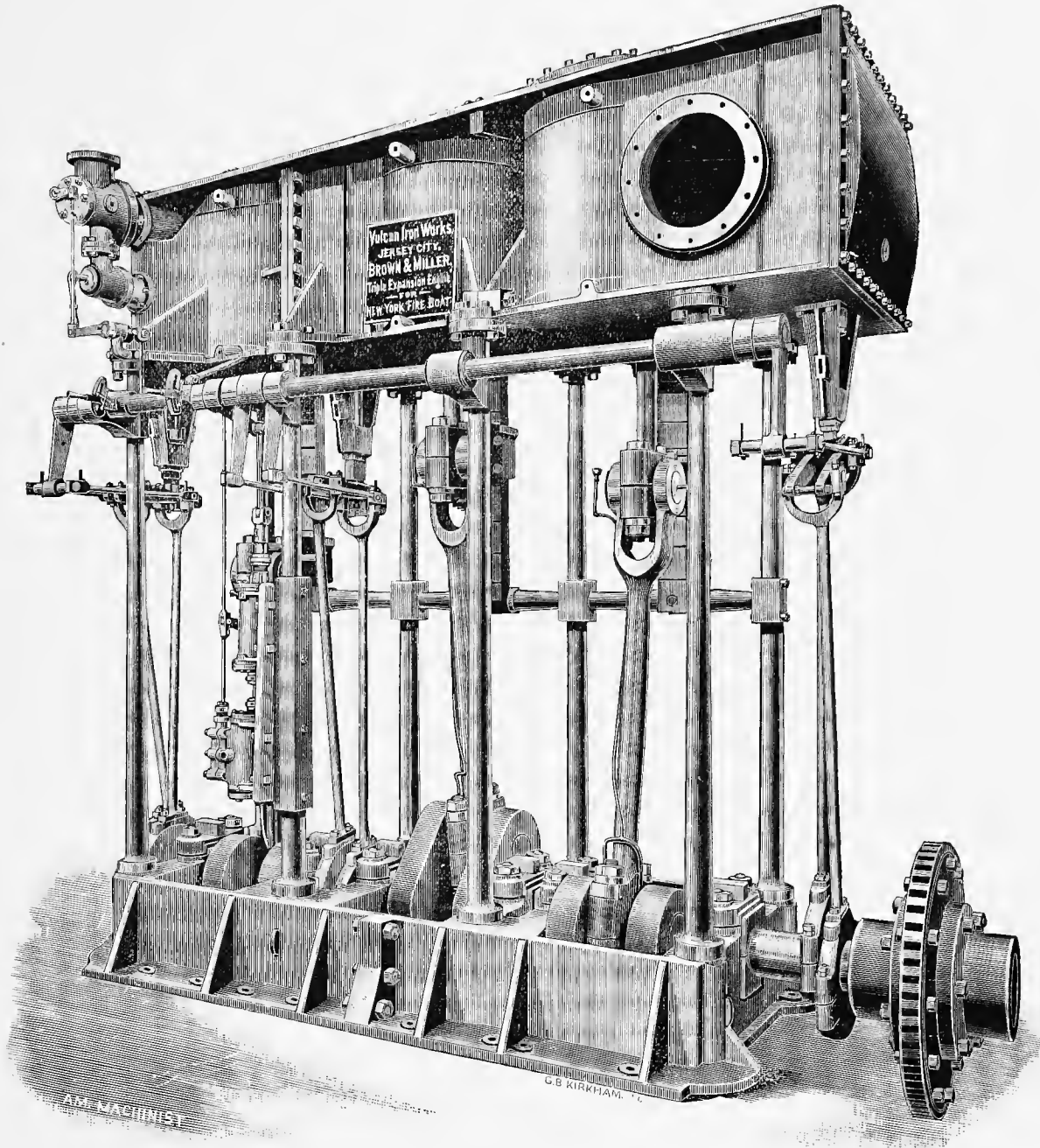
TRIPLE-EXPANSION ENGINE OF THE FIRE BOAT NEW YORKER.
